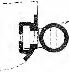
Fig. 3800. Plan. CATCH FOR PULLMAN VESTIBULE GATE.
